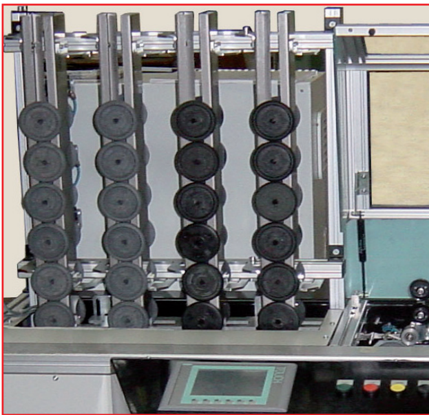
Modular bobbin magazine rack holds up to 40 empty bobbins and allows quick bobbin style changes.
